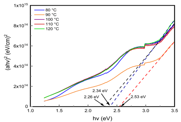
Fig. 7. Bandgap curve of CuSCN samples annealed at different temperatures, ranges between 80 °C to 120 °C
