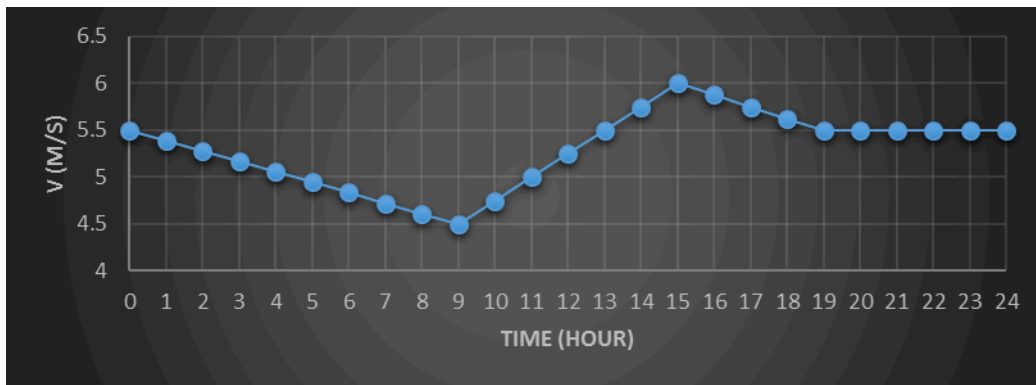
Fig. 5. Distribution of daily wind speed at turbine height used for the turbine power output [11].
