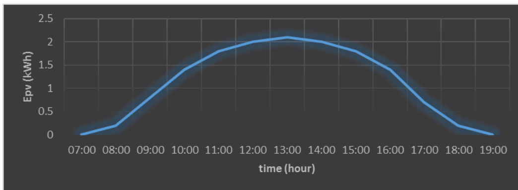
Fig. 6. Distribution of hourly photovoltaic energy generation [12].
