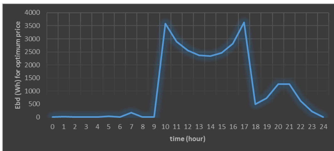
Fig. 9. Simulation results for hourly variations of power flow into the balance boundary of the building through battery storage in case I
