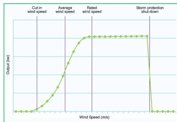
Fig. 2. Idealized wind turbine power curve [7].
