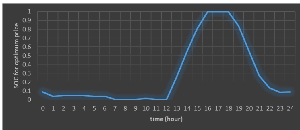
Fig. 11. Simulation results for hourly variations of battery state of charge (SOC) in case I.
