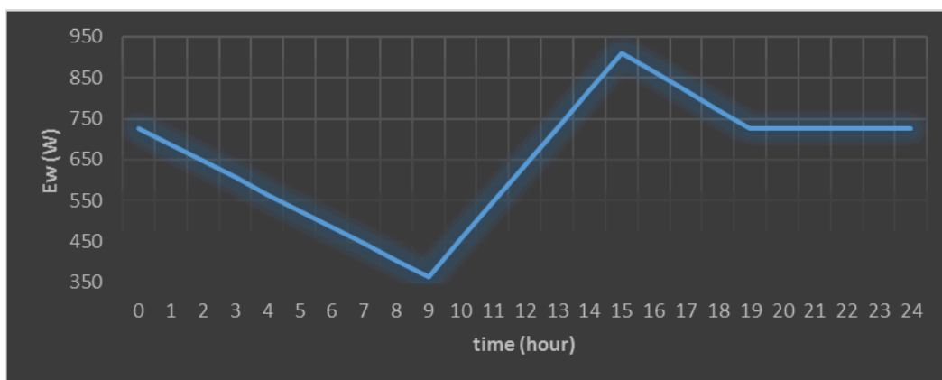
Fig. 8. Distribution of daily wind turbine power used in the model.
