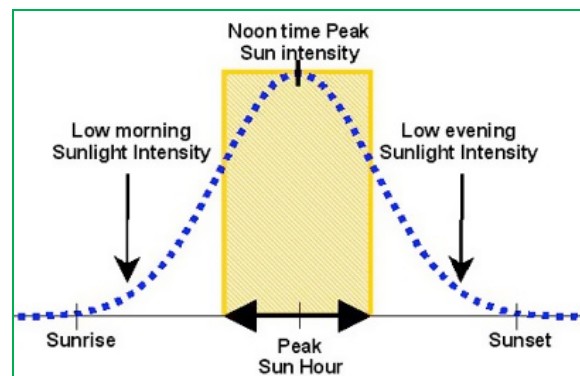
Fig. 2. Typical electricity PV generation profile [6].
