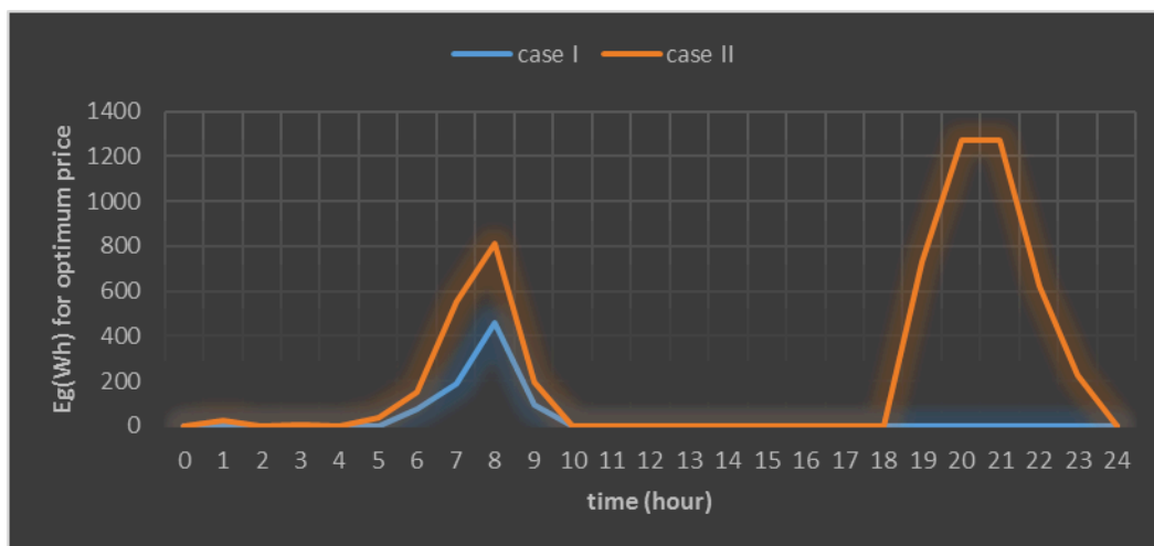
Fig. 10. Simulation results for hourly variations of power flow into the balance boundary of the building through electricity grid in cases I and II.
